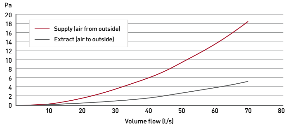
Performance data for double airbrick (code 905) with adapter (977)
