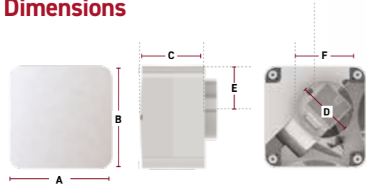
Measured in mm A: 170 B: 170 C: 110 D: 99 E: 72 F: 69
