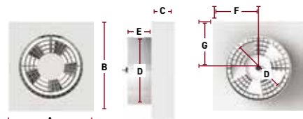
Measured in mm A: 212 B: 227 C: 50 D: 155 E: 53 F: 102.5 G: 110
