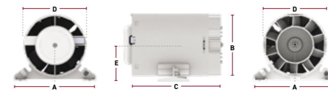
Measured in mm A: 130 B: 107 C: 155 D: 99 E: 57.5
