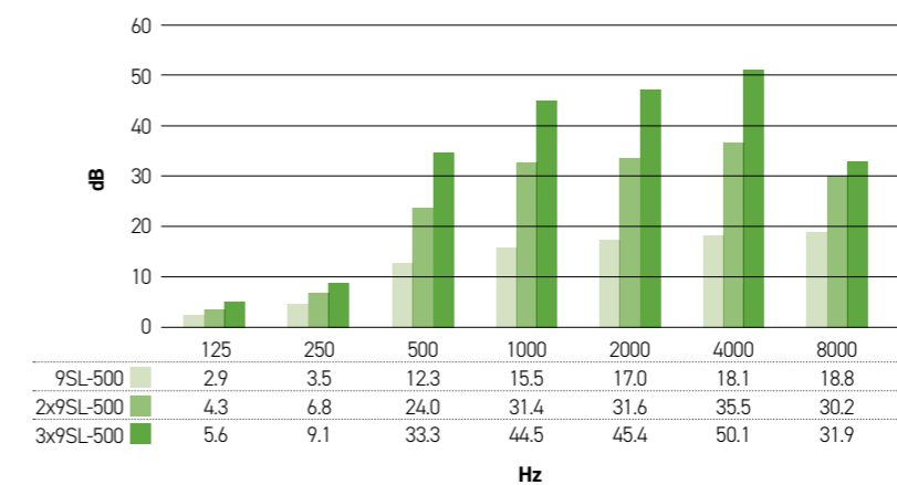
Octave Band Insertion Loss - 9SL-500
