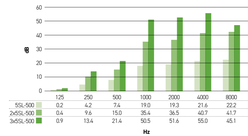
Octave Band Insertion Loss - 5SL-500
